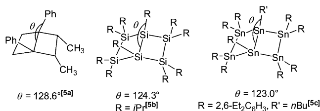
Scheme 2. Selected Group 14 element bicyclo[2.2.0]hexane derivatives.
